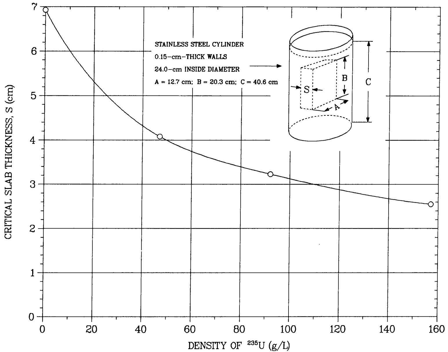
Fig. 26. Critical thicknesses of 12.7- by 20.3-cm U(93) metal slabs immersed in 24-cm-diam \text{U}(93)\text{O}_2(\text{NO}_3)_2 solutions at various ^{235}\text{U} densities.
