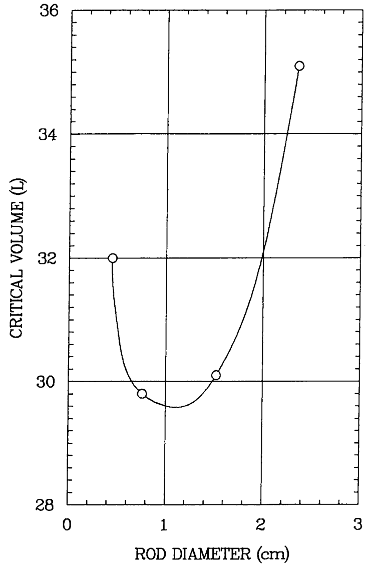
Fig. 20. Critical mass and volume for lattices of U(3.063) metal rods in water. At each rod diameter, the critical volume is that of an equilateral cylinder at optimum lattice spacing, and the critical mass corresponds.
