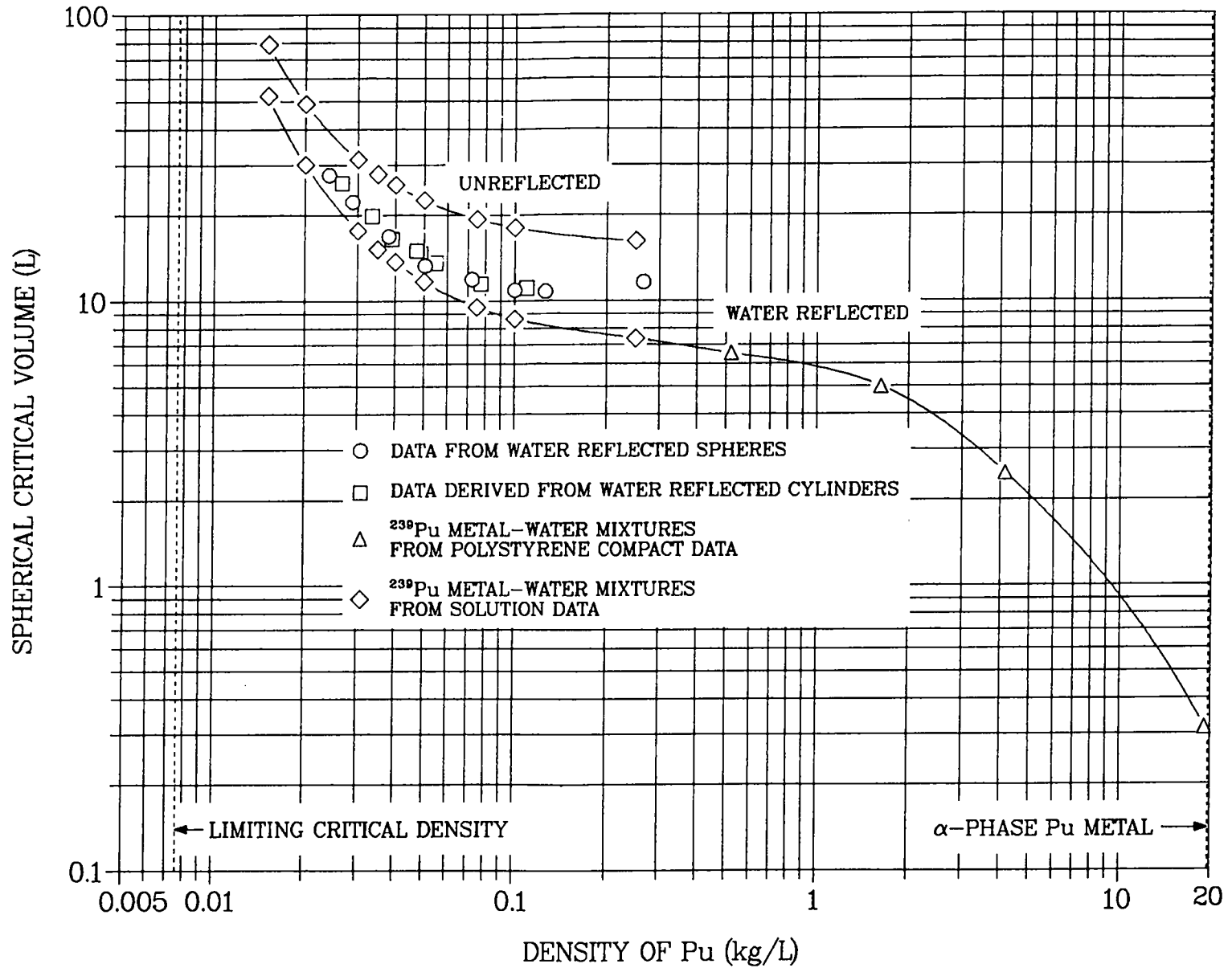
Fig. 32. Critical volumes of homogeneous water-moderated plutonium spheres. The points suggesting an intermediate curve apply to water-reflecting Pu (NO 3 ) 4 solution with 1 N HNO 3 and 3.1% 240 Pu content of the plutonium.
