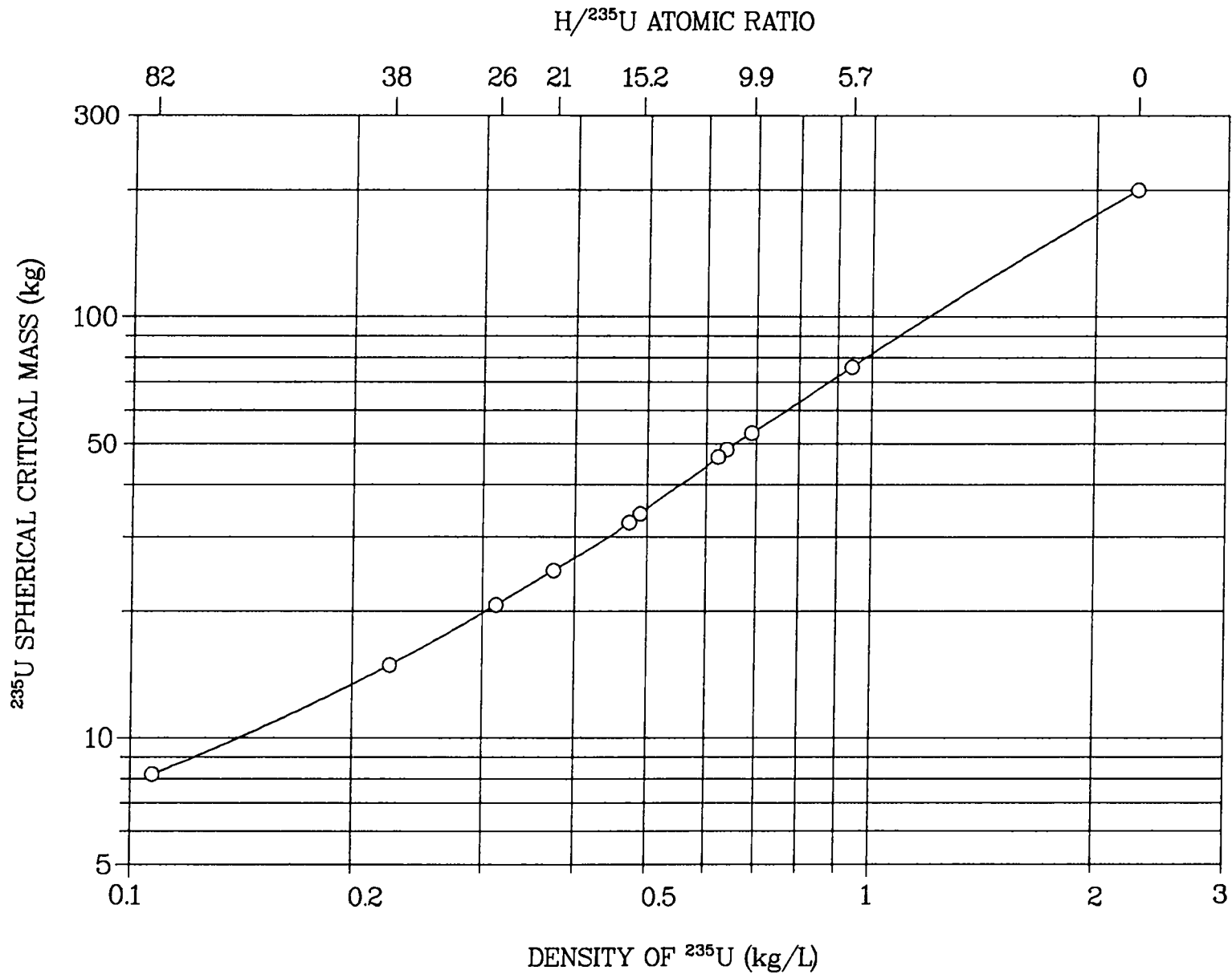
Fig. 3. Critical mass of U(93) as liquid UF_6 -HF at 75^\circ C as a function of ^{235}U density. The system was contained in a water-reflected 0.4-cm-thick Monel sphere.
