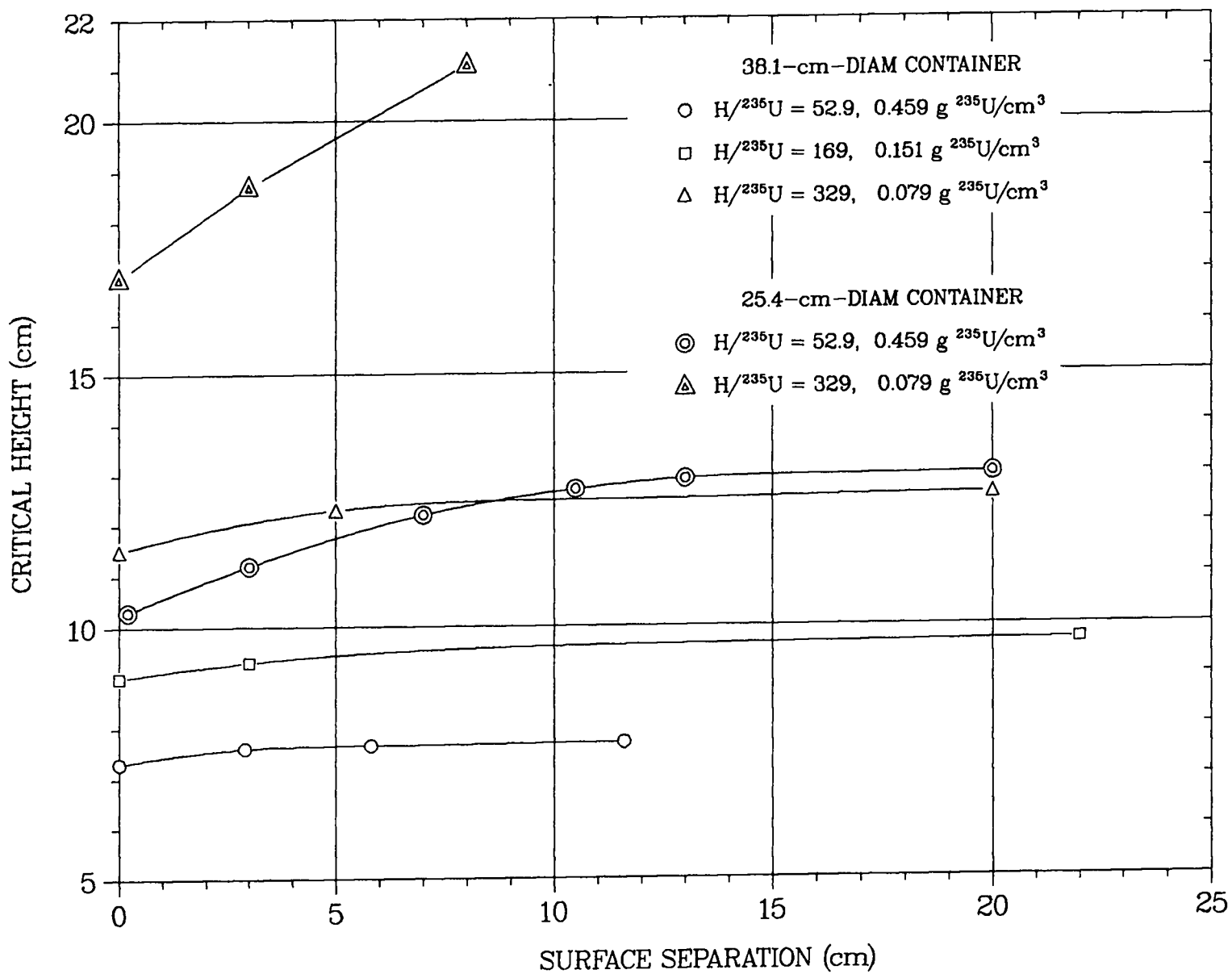
Fig. 50. Common critical height of two interacting U(93.4)O_2F_2 solution cylinders in water. Aluminum containers with 0.15-cm walls. Ref. 168.
