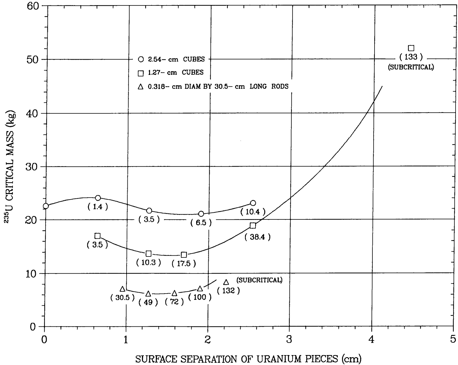
Fig. 21. Critical masses of water-immersed U(94) metal lattices as functions of spacing between units. Mean H/^{235}\text{U} ratios are in parentheses.
