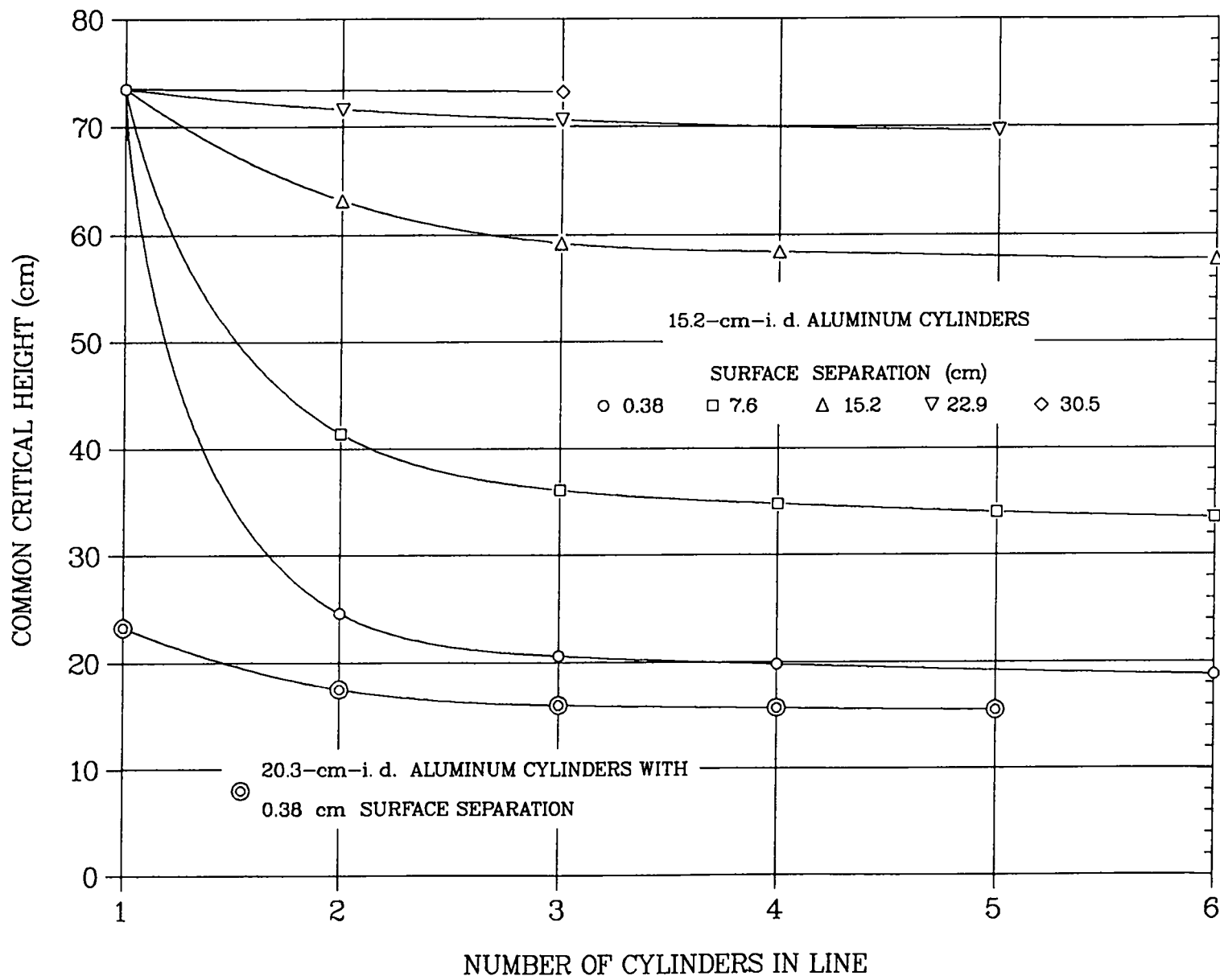
Fig. 51. Common critical height of interacting in-line U(93.4)O_2F_2 solution cylinders in water, H/^{235}U = 44.3 , 0.533 \text{ g } ^{235}U/\text{cm}^3 . Aluminum containers with 0.15-cm walls. Ref. 33.
