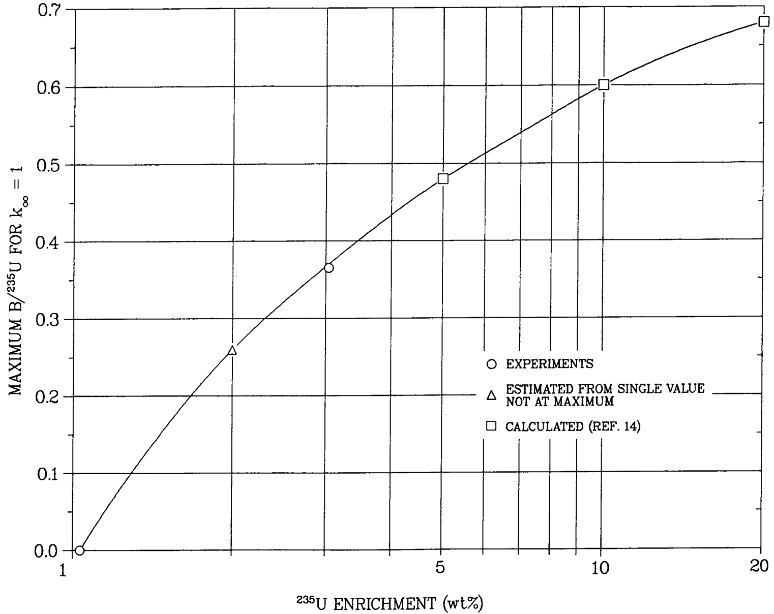
Fig. 41. Maximum boron-to-uranium atomic ratios required for k_{\infty} = 1 vs ^{235}\text{U} enrichment in homogeneous hydrogen-moderated uranium.
