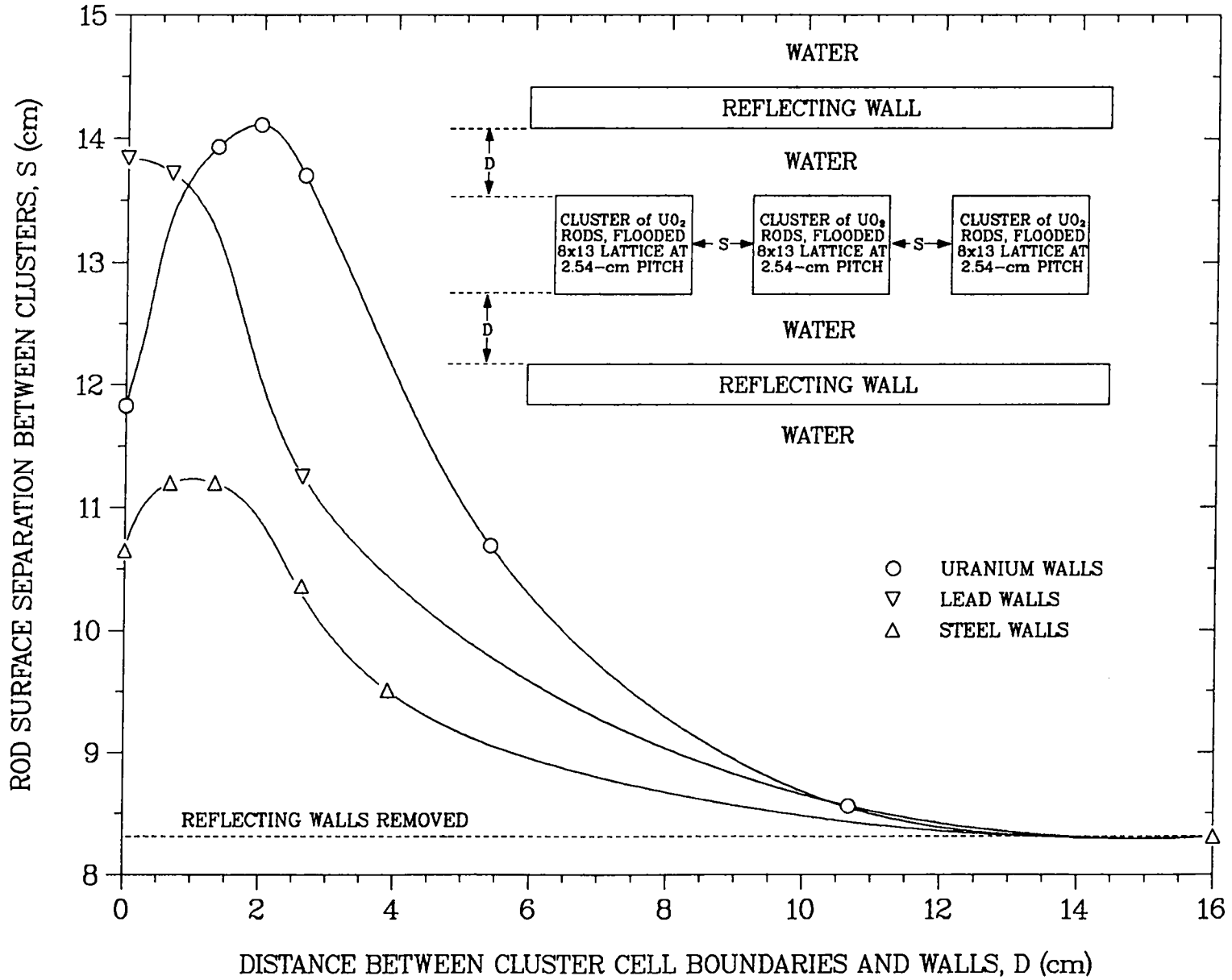
Fig. 73. Critical separations of U(2.35)O_2 rod clusters in water as functions of distance to reflecting walls of steel, lead, or depleted uranium; clusters were at near-optimum moderation.
