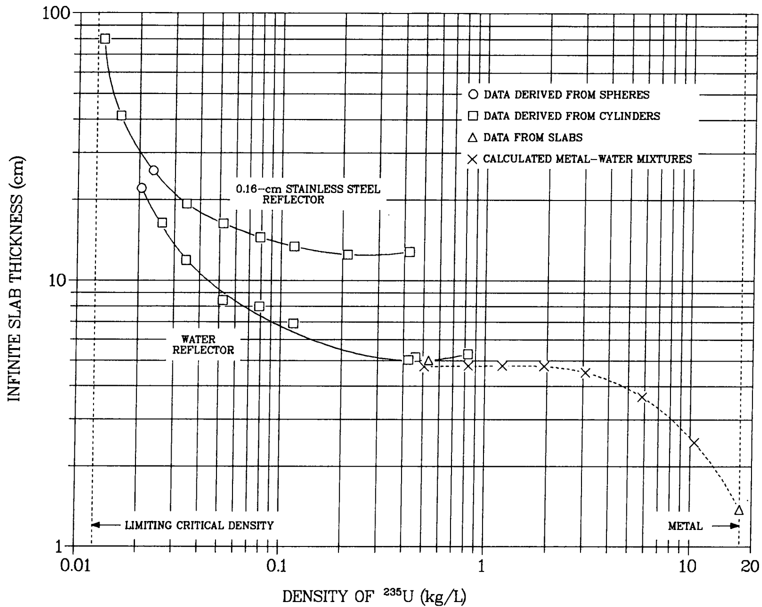
Fig. 13. Estimated critical thicknesses of slabs, infinite in other dimensions, of homogeneous water-moderated U(93.2) . Solution data appear unless indicated otherwise. Unreflected infinite slabs are fictitious.
