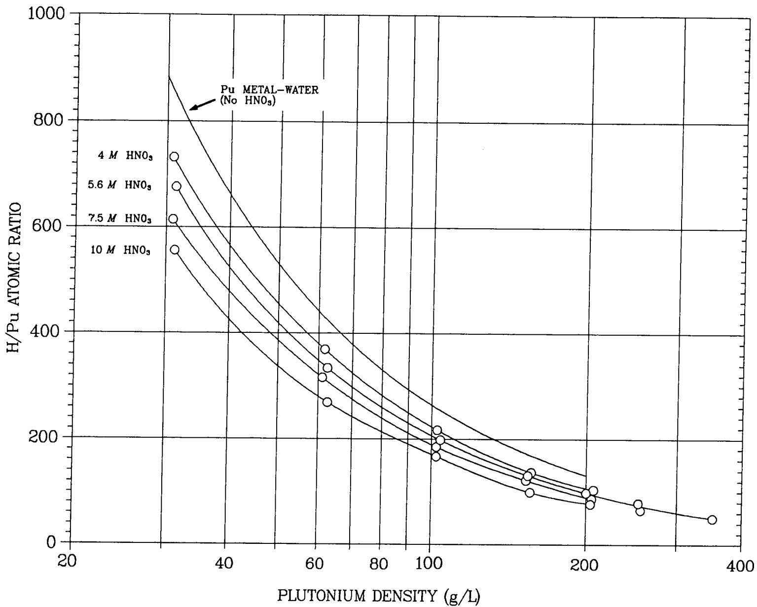
Fig. 29. Atomic ratios H/Pu as functions of plutonium density for \text{Pu}(\text{NO}_3)_4 solutions containing 4 M, 5.6 M, 7.5 M and 10 M \text{HNO}_3 , and for idealized plutonium-water mixtures.
