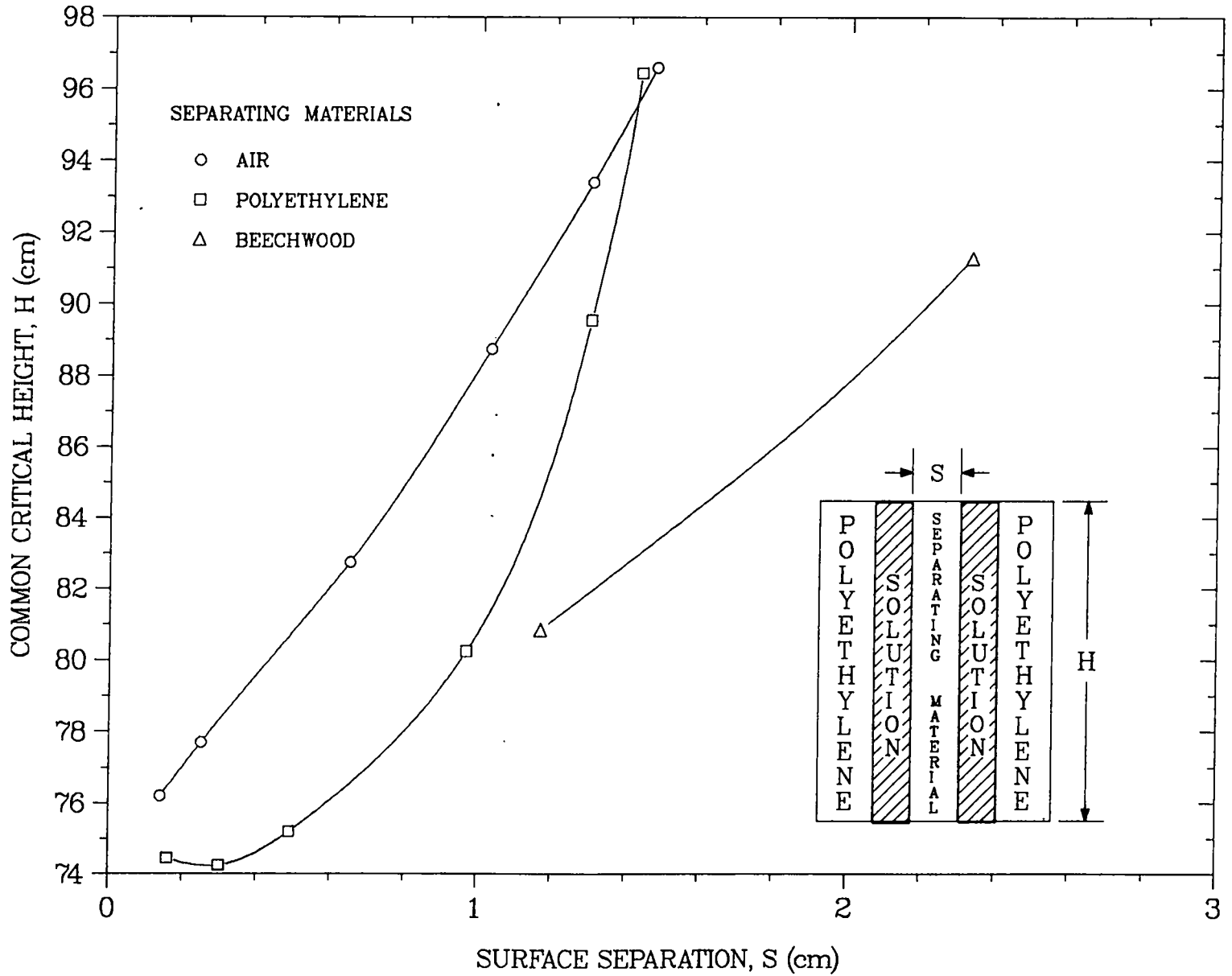
Fig. 66. Common critical height of two parallel U(30.45)O_2F_2 solution slabs with thick polyethylene reflectors on outer faces and separated by air, polyethylene, or beechwood; H/^{235}U = 214, 0.117 \text{ g } ^{235}U/\text{cm}^3 solution. Slabs 120-cm wide by 6.1-cm thick.
