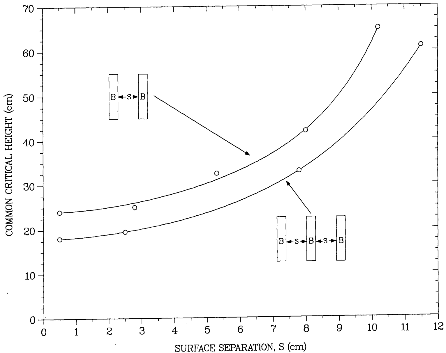
Fig. 59. Common critical heights of two and three parallel U(93.2)O_2F_2 solution slabs in water, H/235 = 337 , 0.076 \text{ g } ^{235}\text{U}/\text{cm}^3 . Aluminum containers with 0.32-cm-thick walls and 120.6-cm-wide by 7.6-cm-thick inside dimensions. Reflection consisted of immersion to height of solution.
