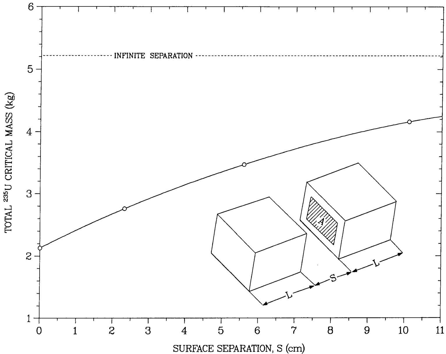
Fig. 67. Total critical mass of two identical U(30.14)O_2 -paraffin parallelepipeds with external polyethylene reflection and separated by air, H/^{235}U = 81.8 , 0.331 \text{ g } ^{235}\text{U}/\text{cm}^3 .
