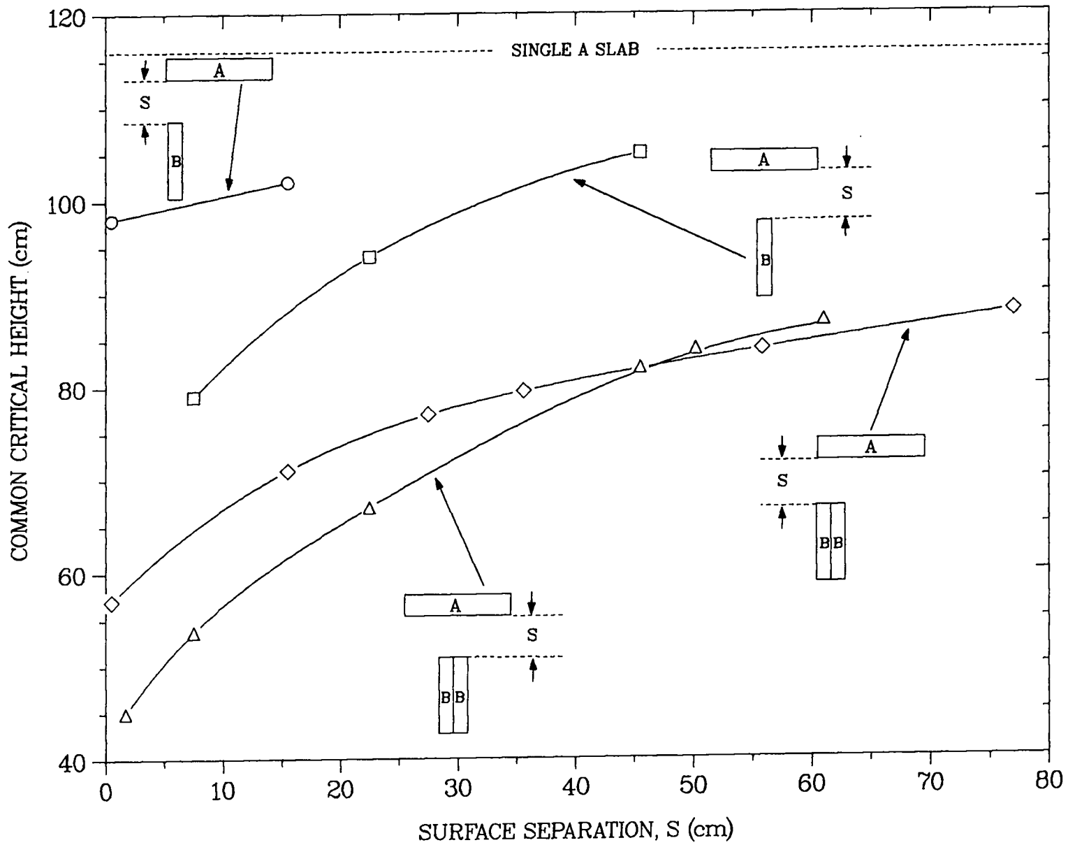
Fig. 61. Common critical heights of pairs of perpendicular U(93.2)O_2F_2 solution slabs in air; H/^{235}U = 325 , 0.079 \text{ g } ^{235}U/\text{cm}^3 solution; 0.32-cm-thick aluminum containers.
