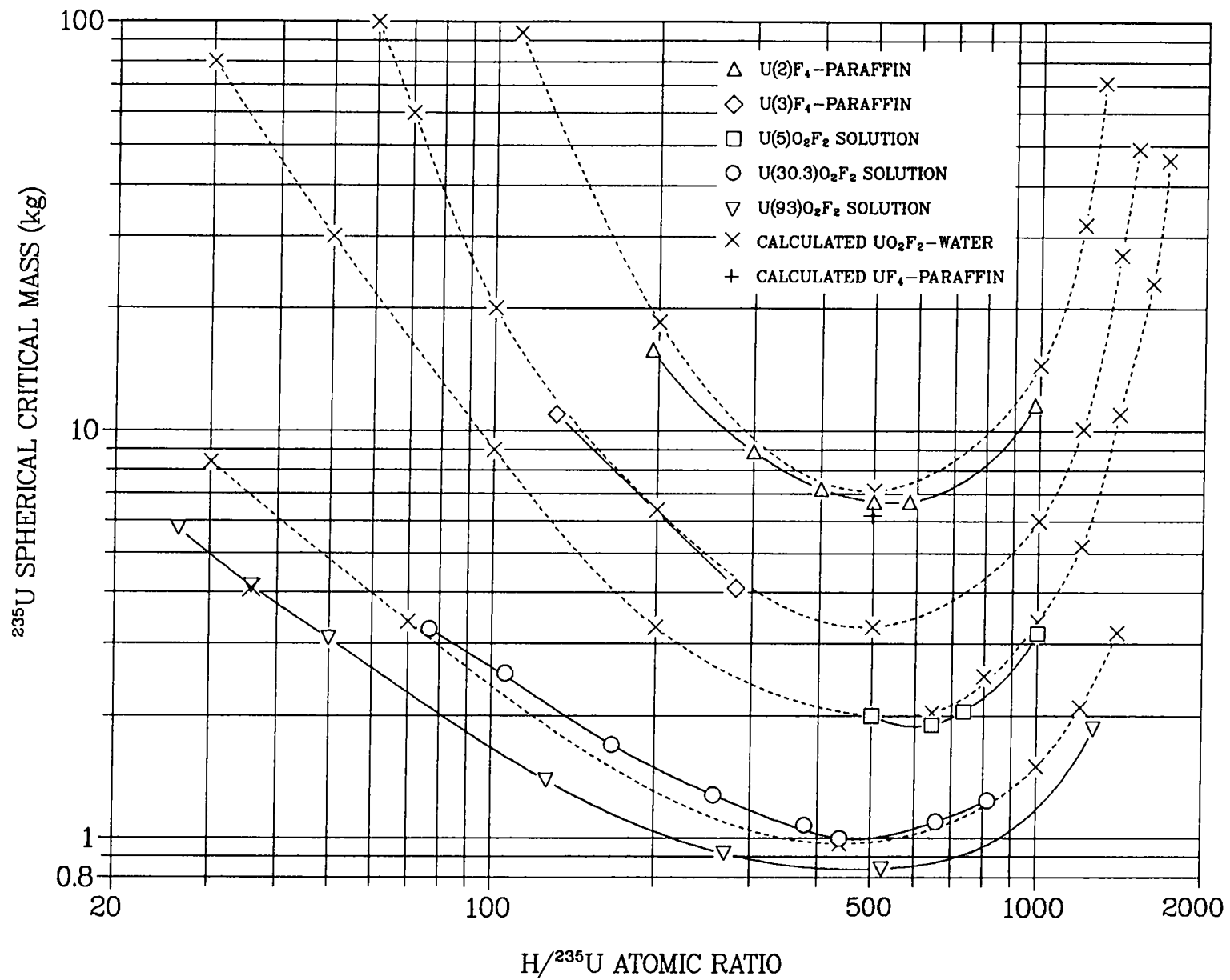
Fig. 14. Critical masses of water-reflected spheres of hydrogen-moderated U(93), U(30.3), U(5.00), U(3.00) and U(2.00).
