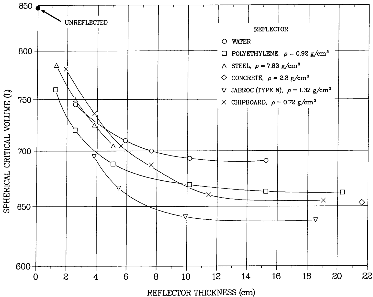
Fig. 44. Spherical critical volumes vs thickness of various reflectors for U(1.42)F_4 -paraffin at H/^{235}U = 422 and \rho(U) = 2.5 \text{ g/cm}^3 . Jabroc is a wood product containing 45% carbon, 6% hydrogen, and 37% oxygen.
