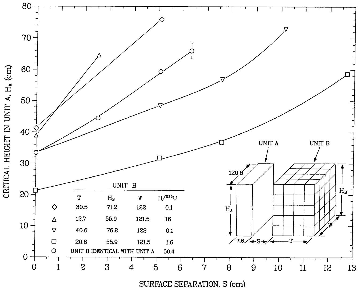
Fig. 64. Critical height of a U(93.2)O_2F_2 solution slab interacting with a parallel slab of U(37)F_4 - CF_2 blocks in air. Unit A was solution in 0.32-cm-thick aluminum container. All dimensions in cm.
