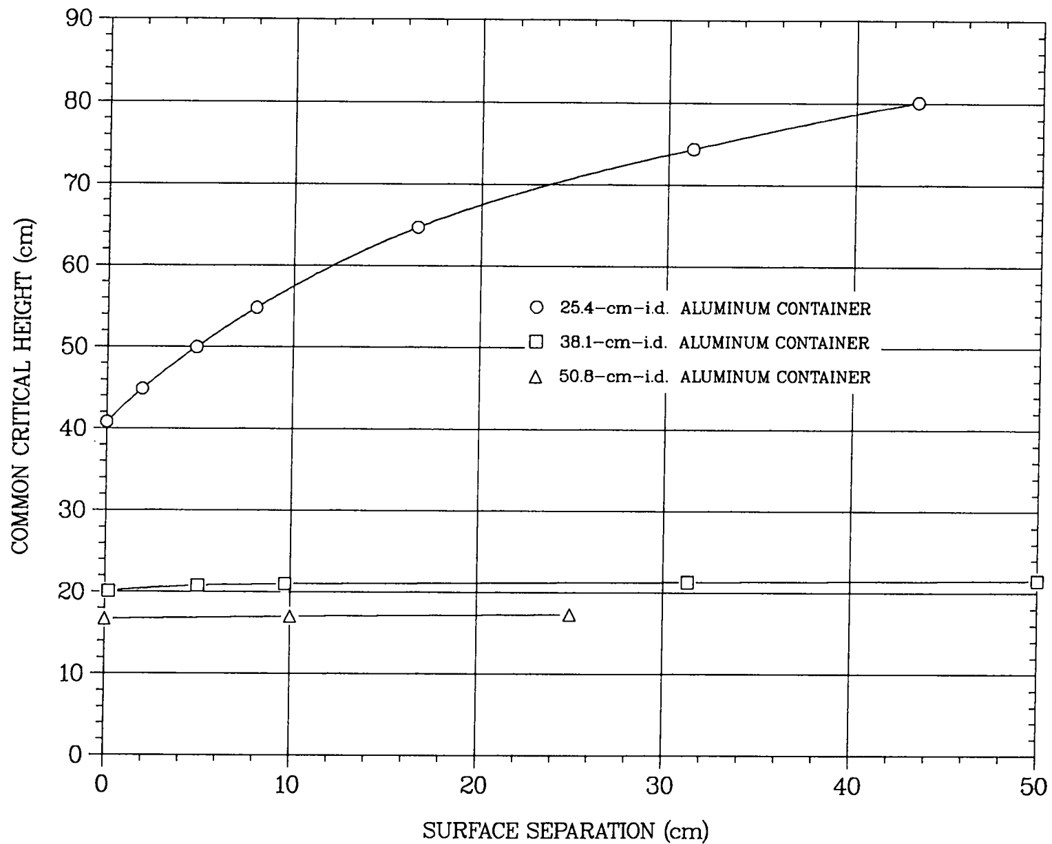
Fig. 53. Common critical height of two interacting U(93.2)O_2F_2 solution cylinders in air, H/^{235}U = 329 , 0.0787 \text{ g } ^{235}\text{U}/\text{cm}^3 ). Ref. 168.
