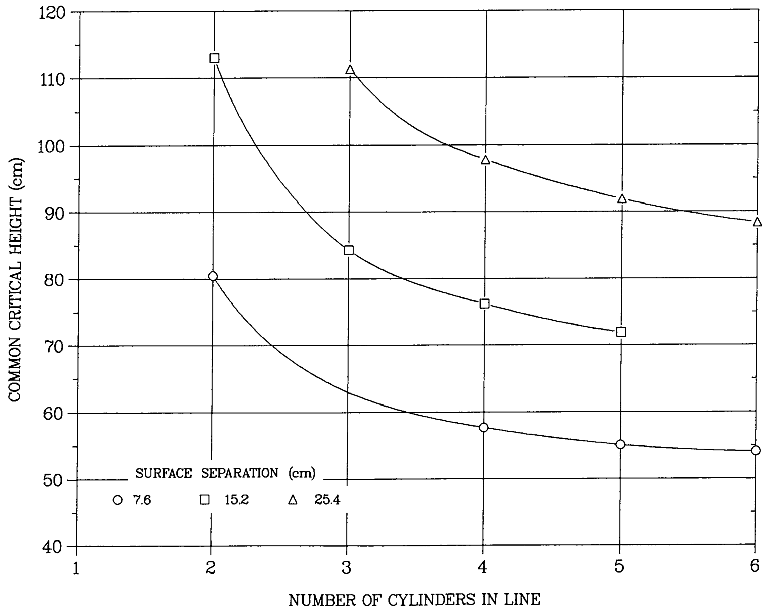
Fig. 54. Common critical height of interacting in-line U(93.2)O_2F_2 solution cylinders in air, H/^{235}U = 297 , 0.087 \text{ g } ^{235}U/\text{cm}^3 , 24.1-cm-i.d. aluminum containers with 0.15-cm-thick walls. Ref. 169.
